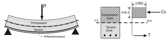
Fig. 1 Flexural Action of Reinforced Concrete Beam
